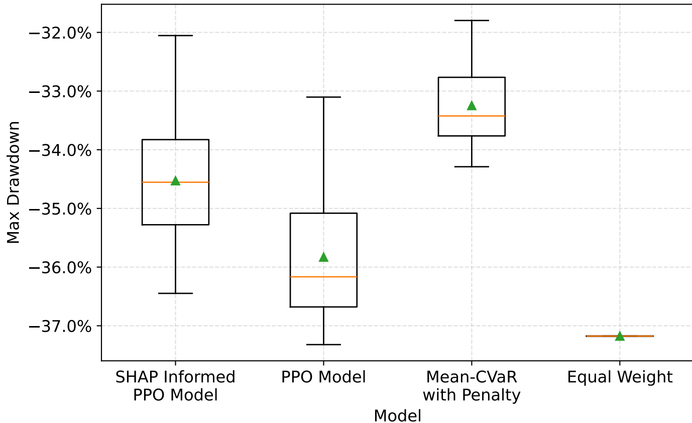
Sector ETFs: MaxDD — Distribution Across 30 Iterations
